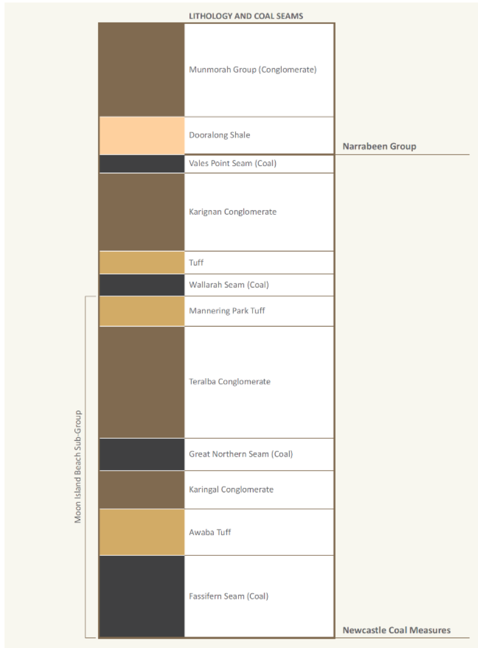
Figure 3.1: General Stratigraphic Column within Colliery Holding area (not to scale)
