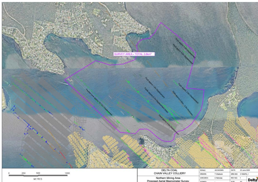
Figure 2.3: Proposed drone aerial magnetic survey over Lake Macquarie for igneous intrusions over the Northern Mining Area
